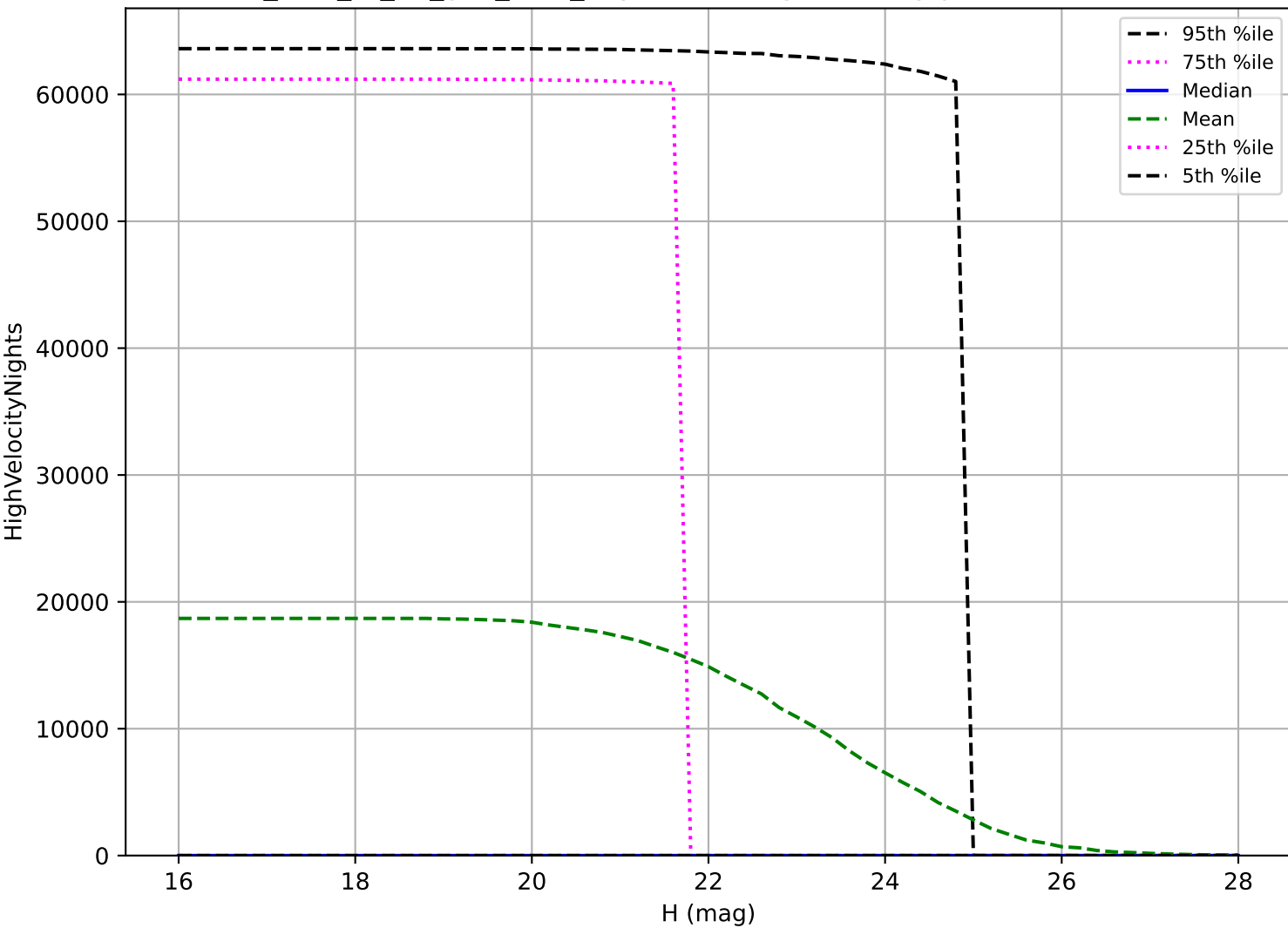
too_elab_r8_d2_griz_v3.4_10yrs: NEO High velocity pair detection loss
