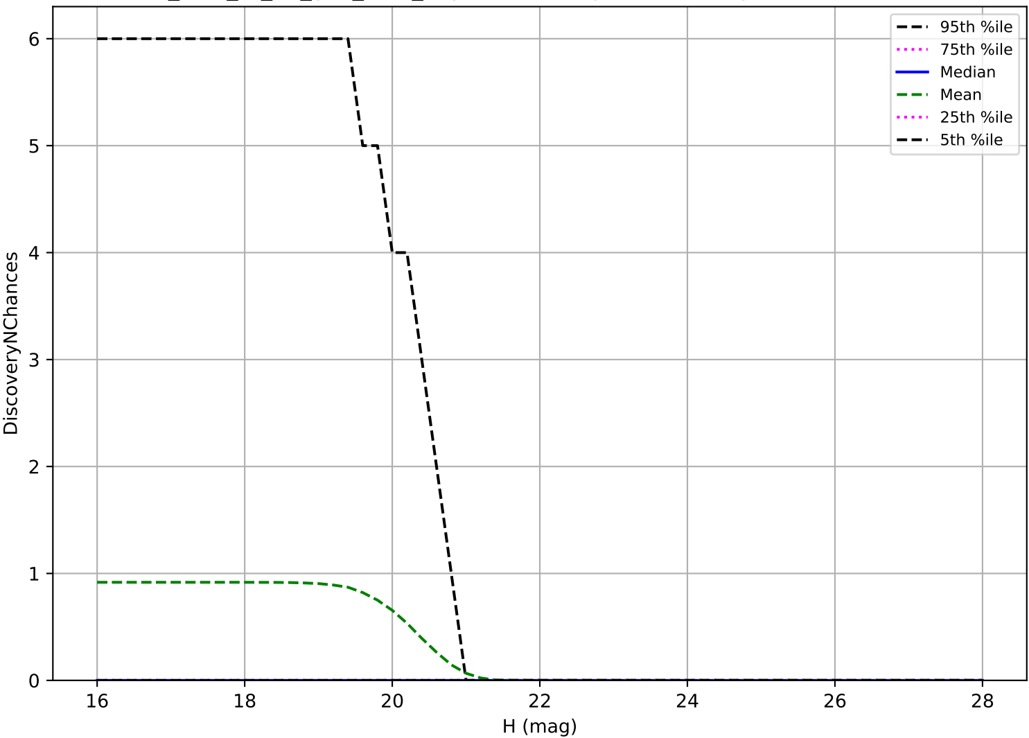
too_elab_r8_d2_griz_v3.4_10yrs: Vatira 3 pairs in 15 nights detection loss
