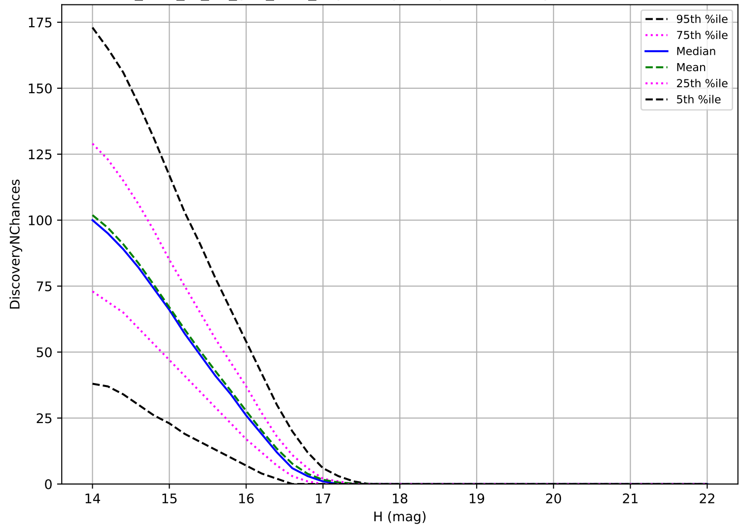
too_elab_r8_d2_griz_v3.4_10yrs: Trojan 3 pairs in 15 nights detection loss
