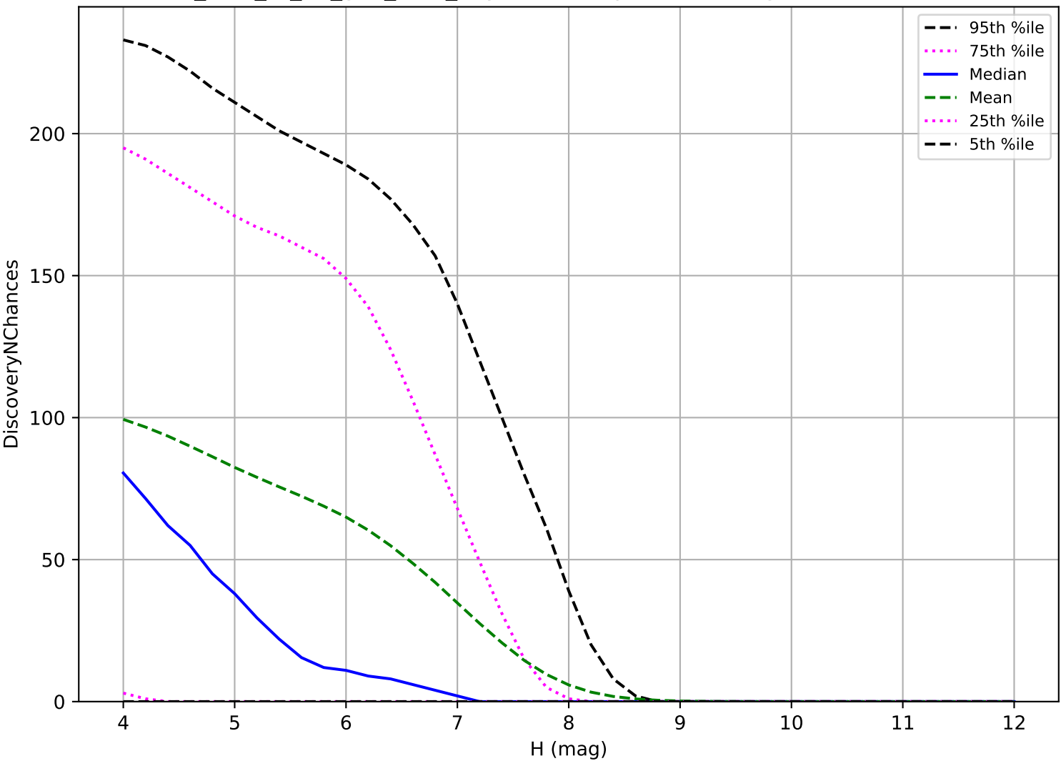
too_elab_r8_d2_griz_v3.4_10yrs: TNO 3 pairs in 15 nights detection loss
