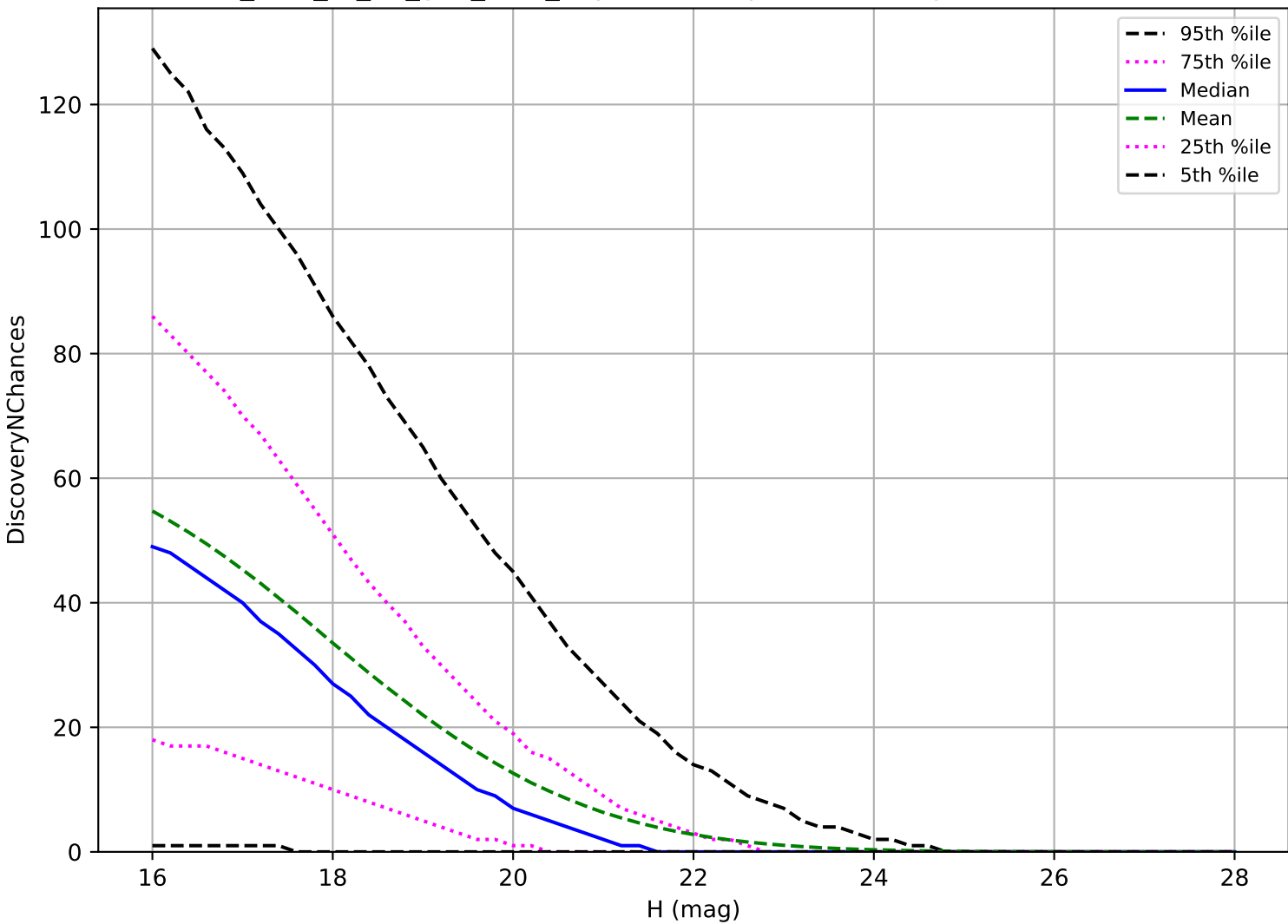
too_elab_r8_d2_griz_v3.4_10yrs: PHA 3 pairs in 15 nights detection loss
