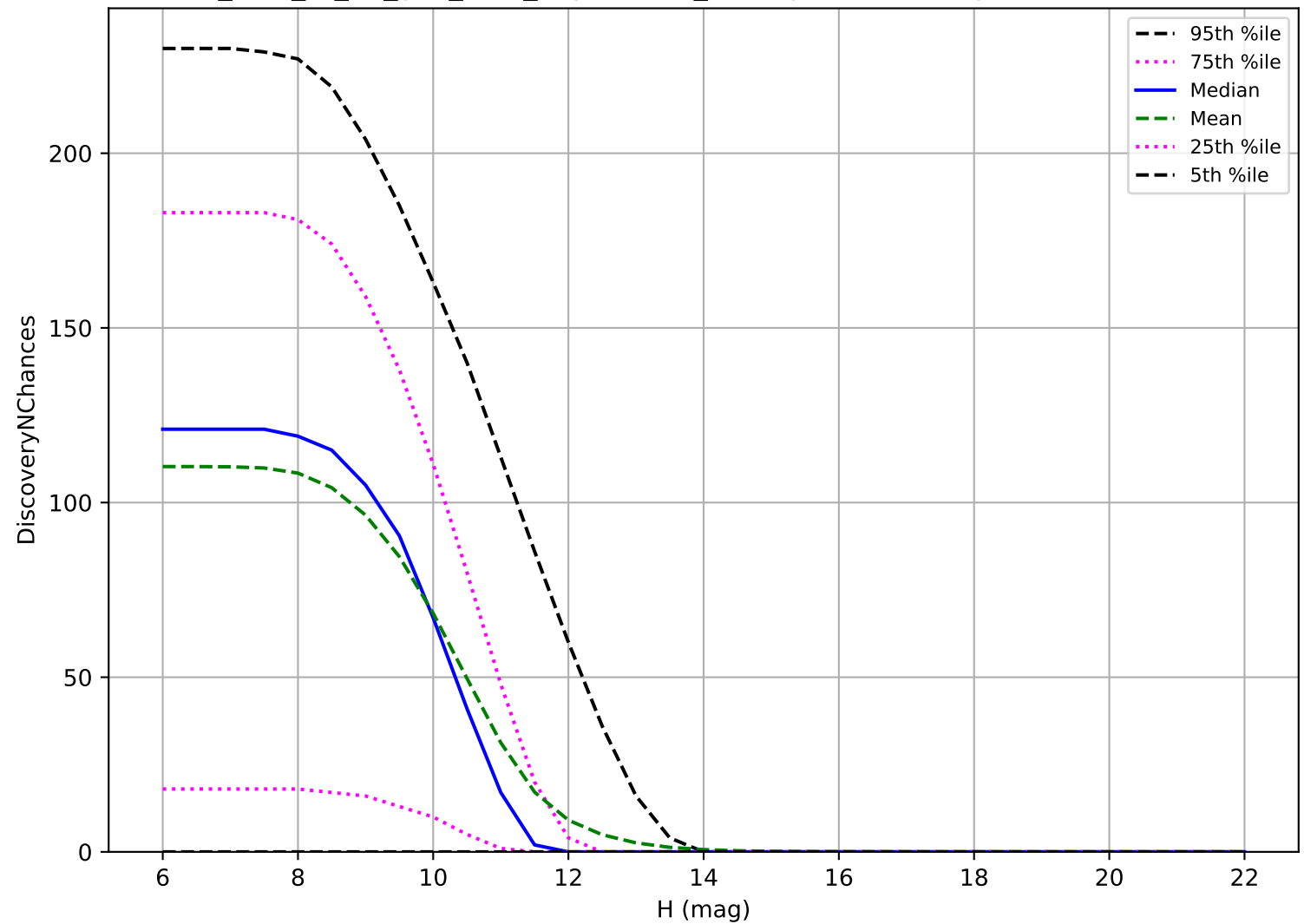
too_elab_r8_d2_griz_v3.4_10yrs: OCC_r20 3 pairs in 15 nights detection loss
