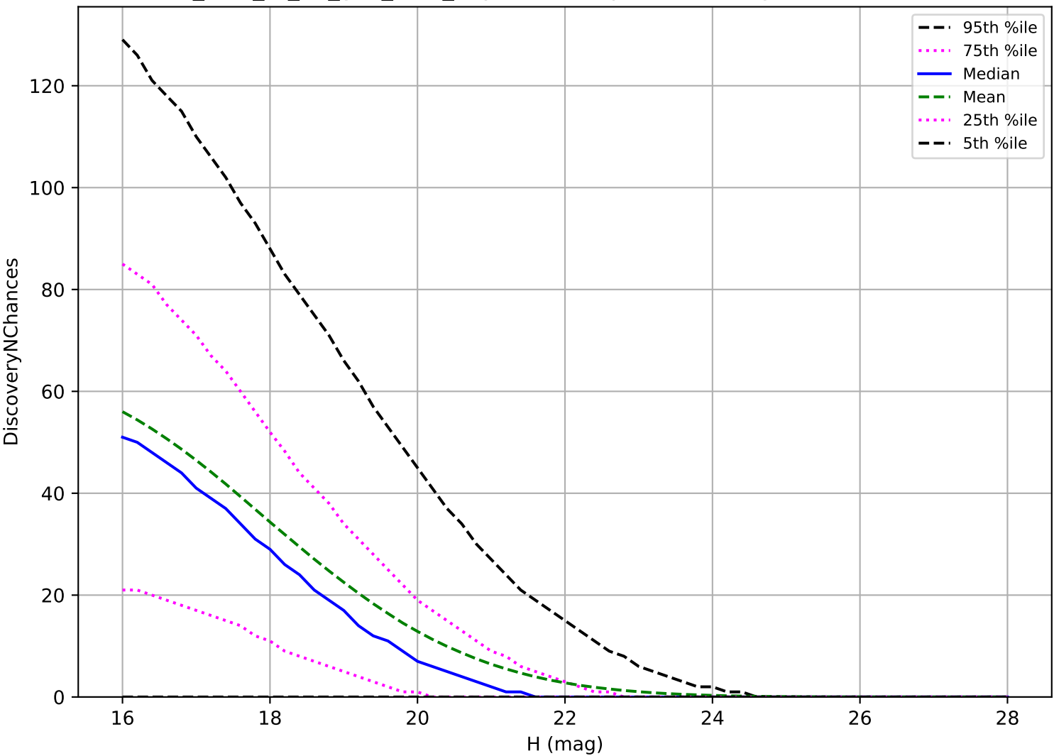
too_elab_r8_d2_griz_v3.4_10yrs: NEO 3 pairs in 15 nights detection loss
