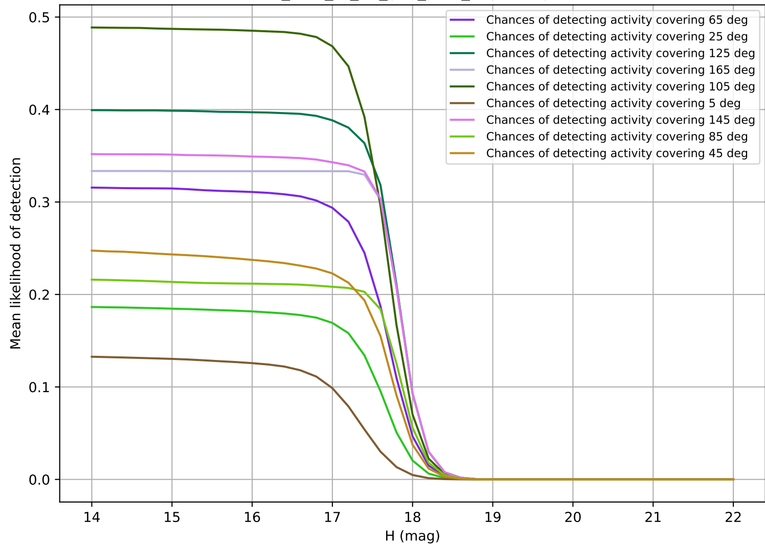
too_elab_r8_d2_griz_v3.4_10yrs Trojan
