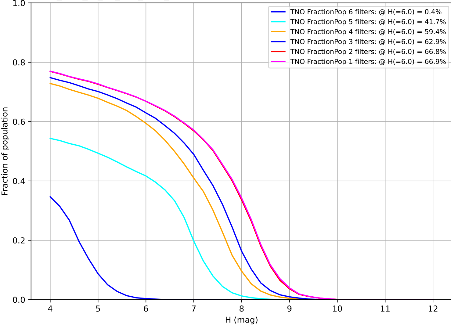
too_elab_r8_d2_griz_v3.4_10yrs: Fraction of population with colors in X filters TNO
