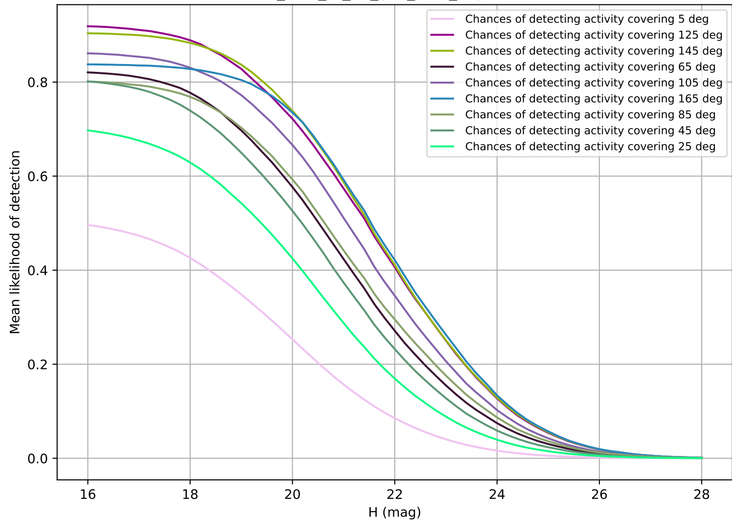
too_elab_r8_d2_griz_v3.4_10yrs PHA
