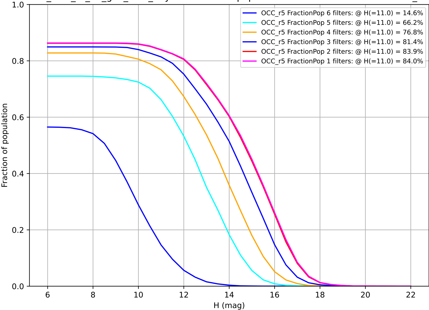
too_elab_r8_d2_griz_v3.4_10yrs: Fraction of population with colors in X filters OCC_r5
