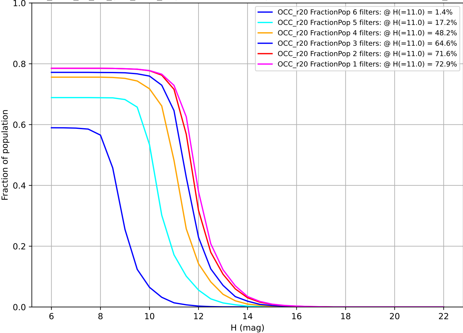
too_elab_r8_d2_griz_v3.4_10yrs: Fraction of population with colors in X filters OCC_r20
