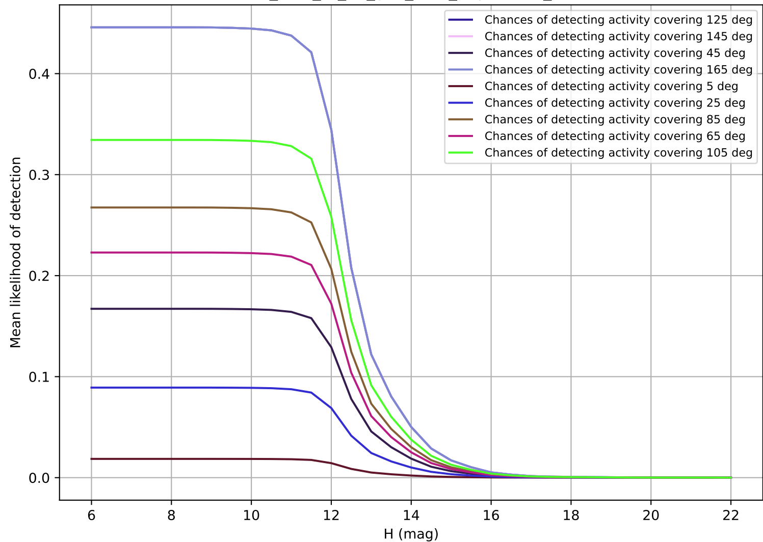
too_elab_r8_d2_griz_v3.4_10yrs OCC_r20
