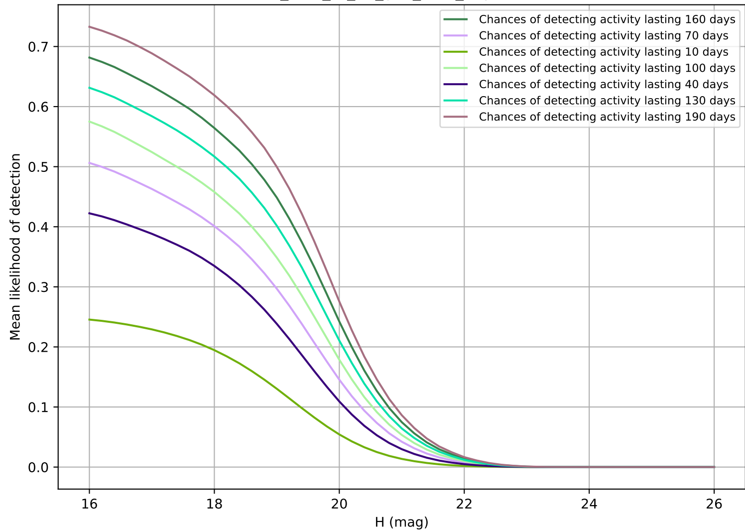
too_elab_r8_d2_griz_v3.4_10yrs MBA
