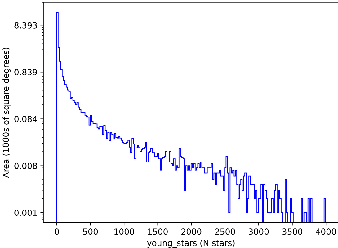
too_elab_r8_d2_griz_v3.4_10yrs : young_stars
