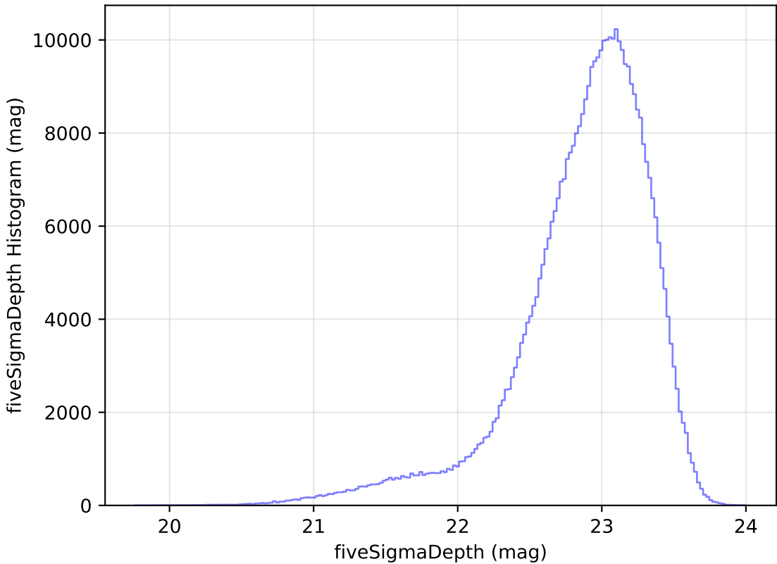
too_elab_r8_d2_griz_v3.4_10yrs z: fiveSigmaDepth Histogram
