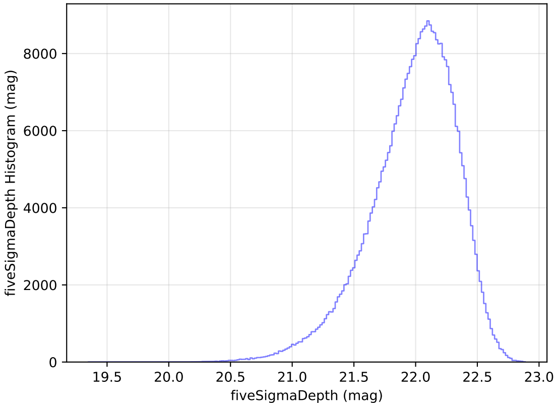
too_elab_r8_d2_griz_v3.4_10yrs y: fiveSigmaDepth Histogram
