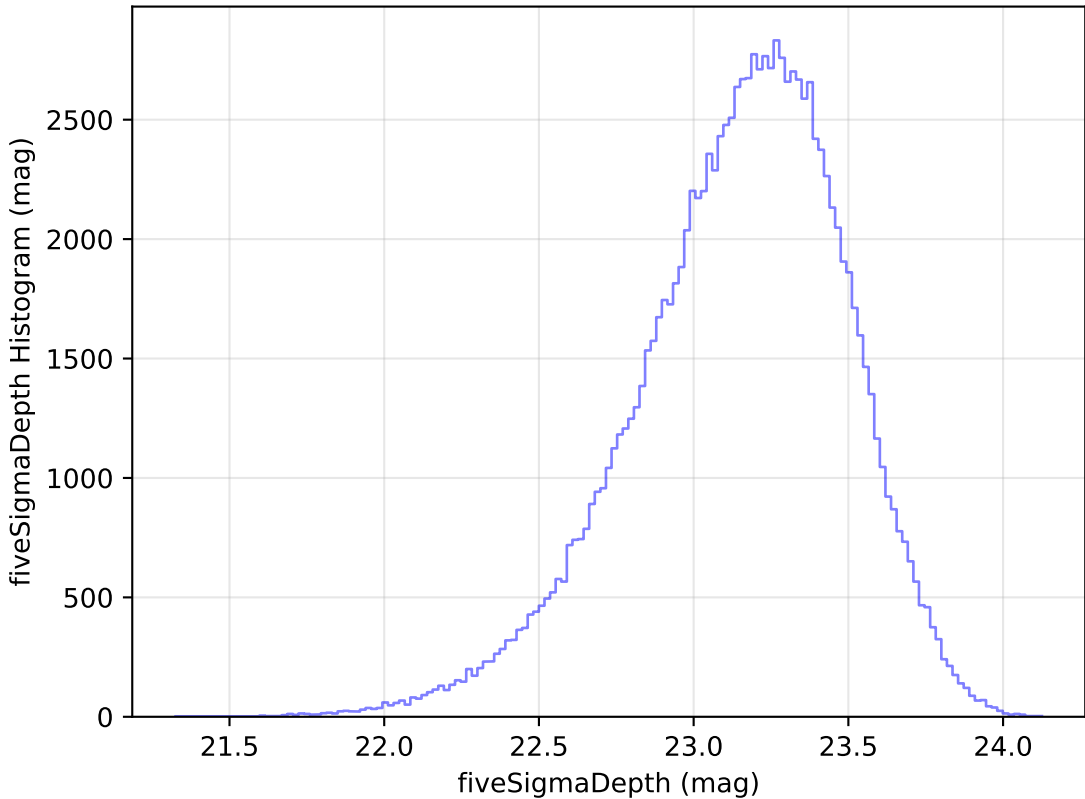
too_elab_r8_d2_griz_v3.4_10yrs u: fiveSigmaDepth Histogram
