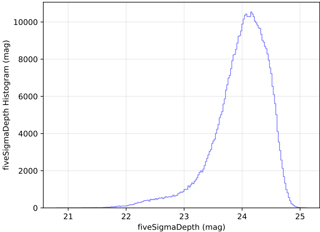
too_elab_r8_d2_griz_v3.4_10yrs r: fiveSigmaDepth Histogram
