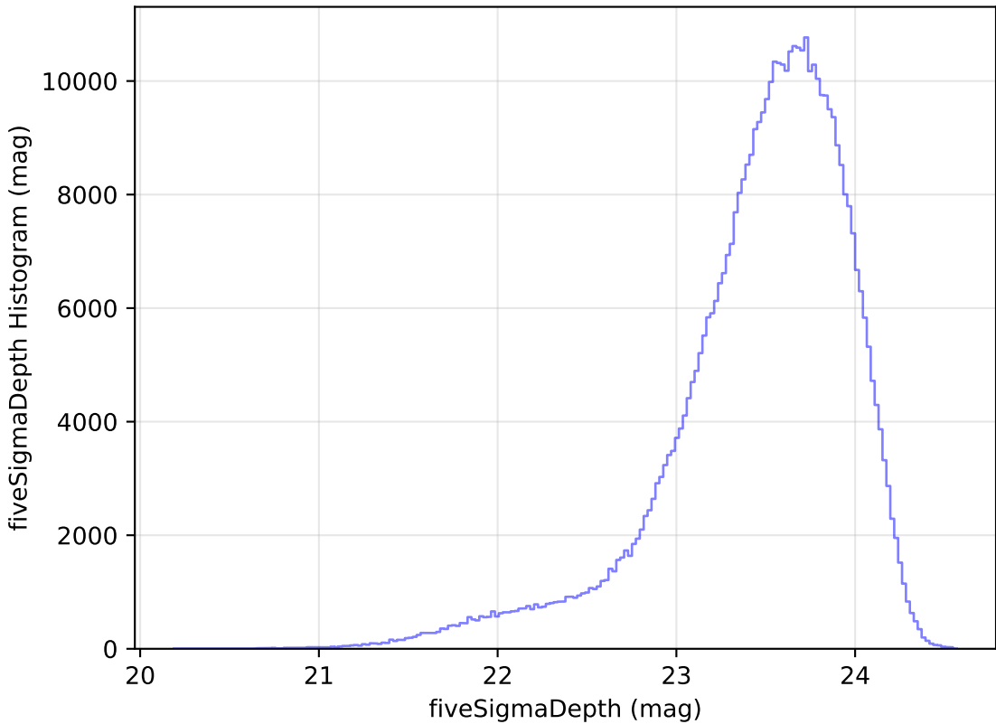
too_elab_r8_d2_griz_v3.4_10yrs i: fiveSigmaDepth Histogram
