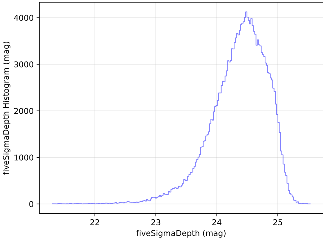
too_elab_r8_d2_griz_v3.4_10yrs g: fiveSigmaDepth Histogram
