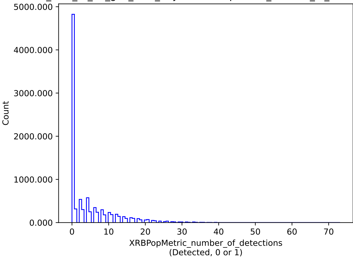
too_elab_r8_d2_griz_v3.4_10yrs : XRBPopMetric_number_of_detections
