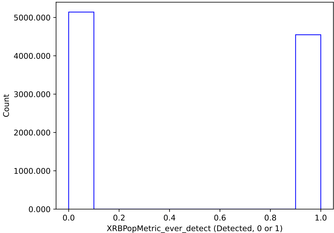
too_elab_r8_d2_griz_v3.4_10yrs : XRBPoMetric_ever_detect
