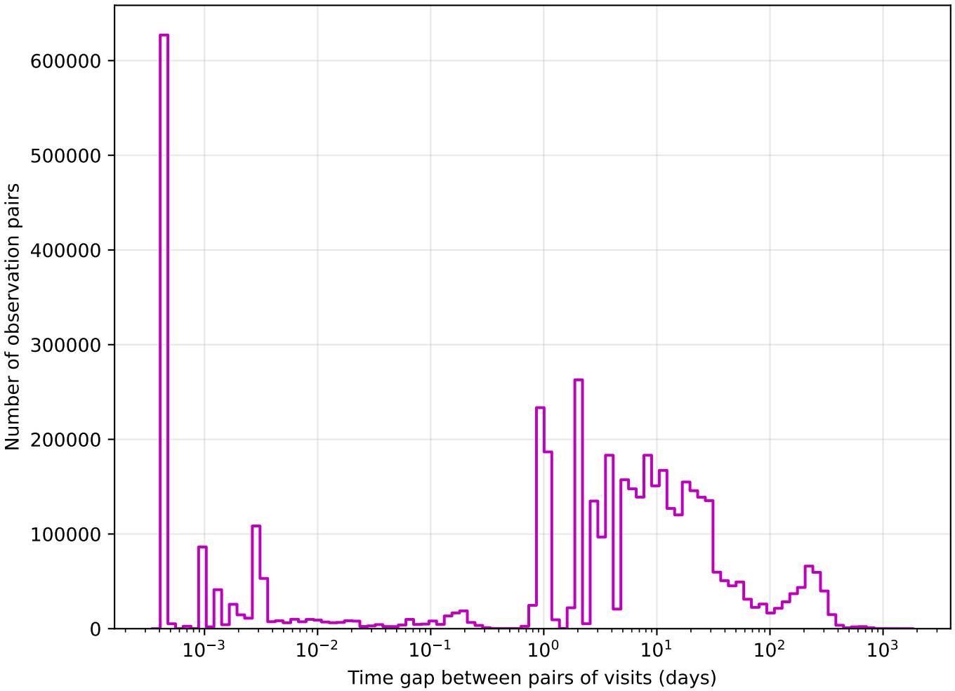
too_elab_r8_d2_griz_v3.4_10yrs z band: Tgaps observationStartMJD
