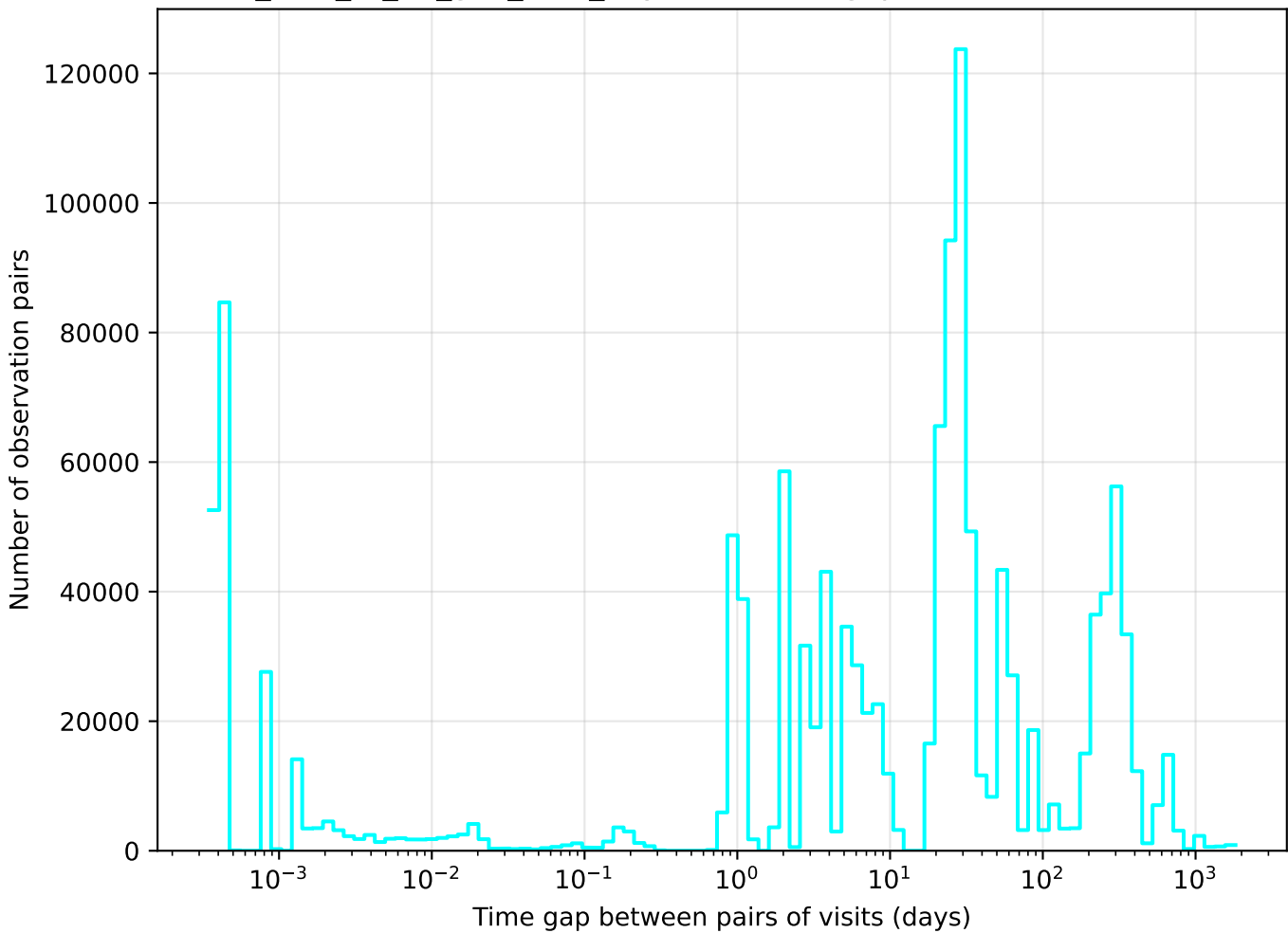
too_elab_r8_d2_griz_v3.4_10yrs u band: Tgaps observationStartMJD
