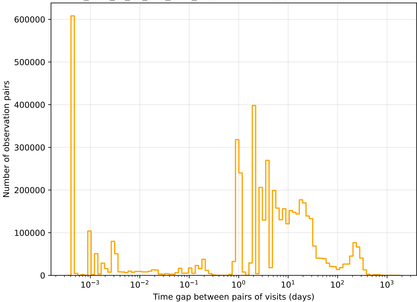
too_elab_r8_d2_griz_v3.4_10yrs r band: Tgaps observationStartMJD
