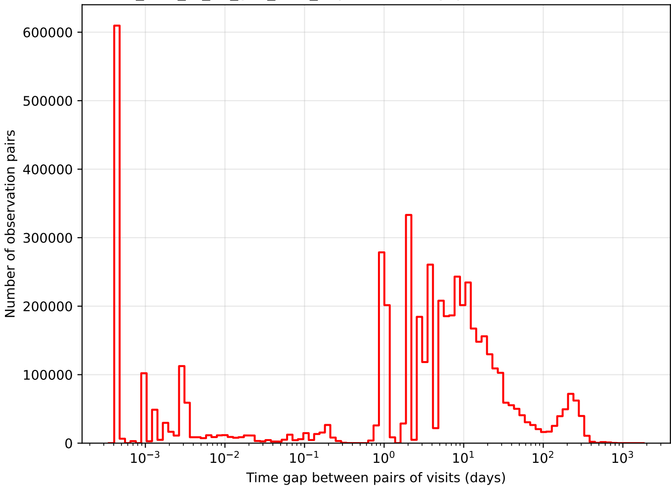
too_elab_r8_d2_griz_v3.4_10yrs i band: Tgaps observationStartMJD
