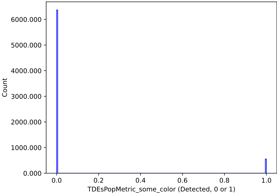
too_elab_r8_d2_griz_v3.4_10yrs : TDEsPopMetric_some_color
