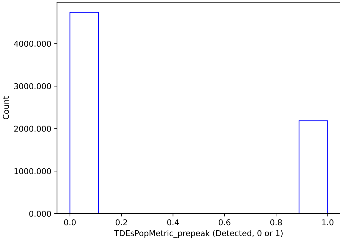
too_elab_r8_d2_griz_v3.4_10yrs : TDEsPopMetric_prepeak
