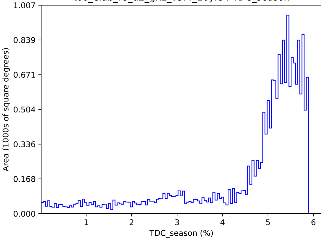
too_elab_r8_d2_griz_v3.4_10yrs : TDC_season
