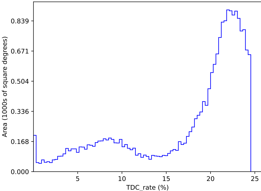
too_elab_r8_d2_griz_v3.4_10yrs : TDC_rate
