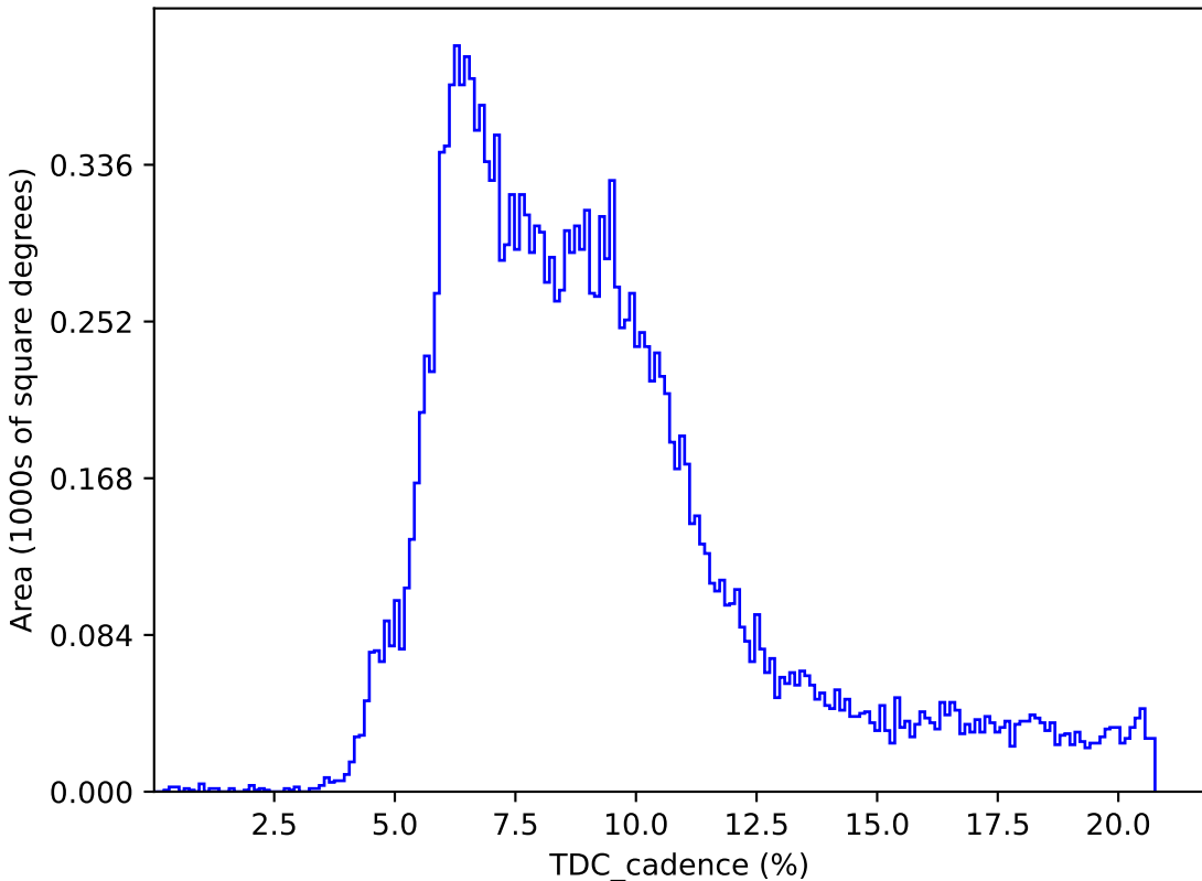
too_elab_r8_d2_griz_v3.4_10yrs : TDC_cadence
