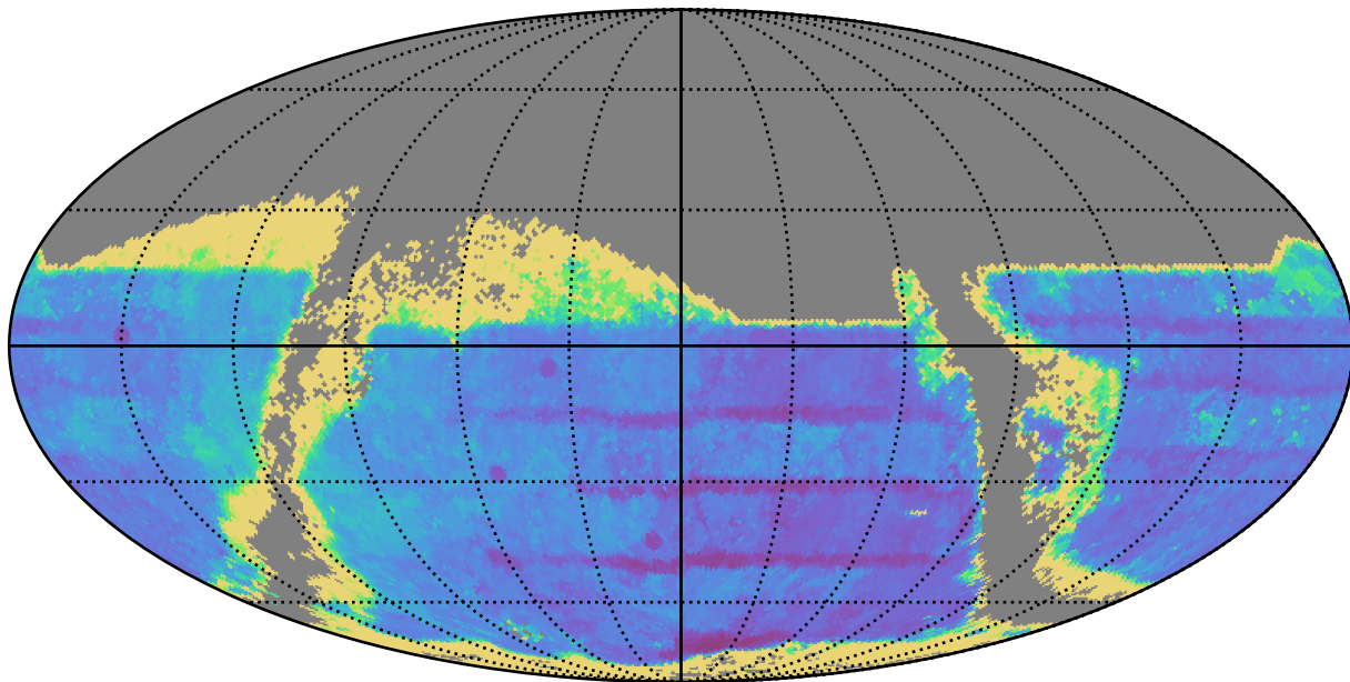
too_elab_r8_d2_griz_v3.4_10yrs : TDC_accuracy
