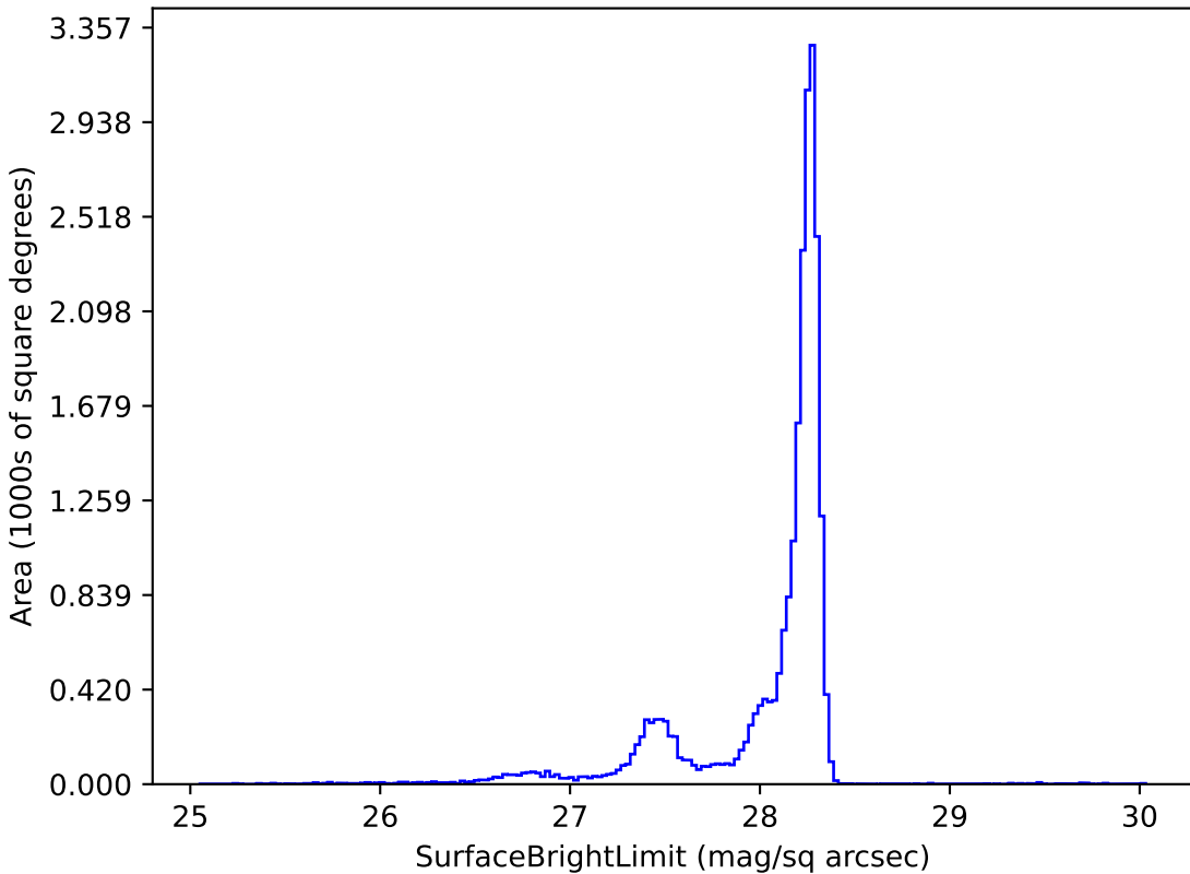
too_elab_r8_d2_griz_v3.4_10yrs y: SurfaceBrightLimit
