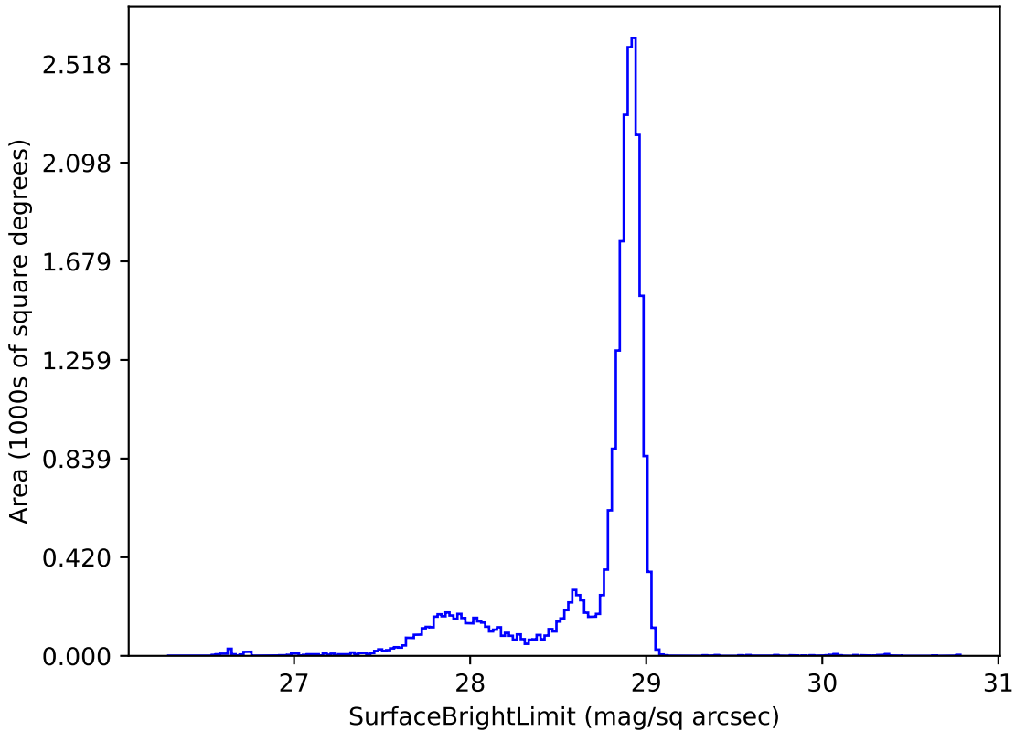
too_elab_r8_d2_griz_v3.4_10yrs u: SurfaceBrightLimit
