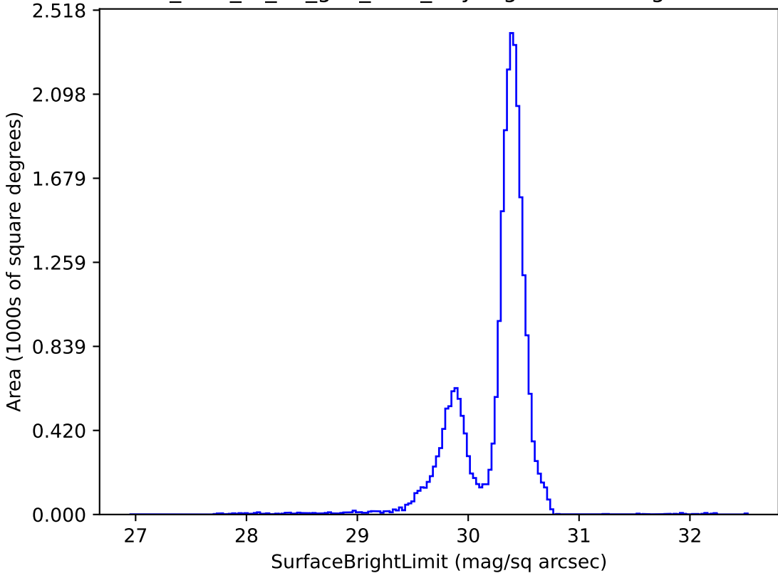
too_elab_r8_d2_griz_v3.4_10yrs g: SurfaceBrightLimit
