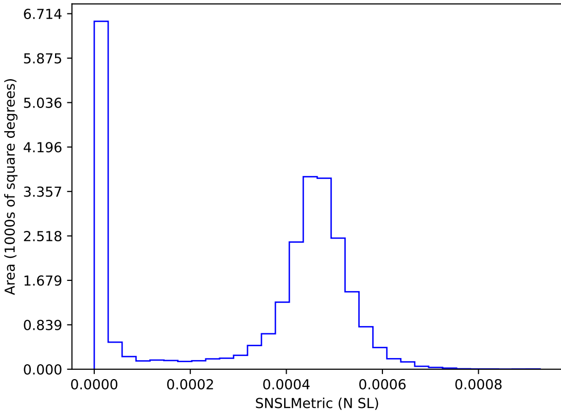
too_elab_r8_d2_griz_v3.4_10yrs : SNSLMetric
