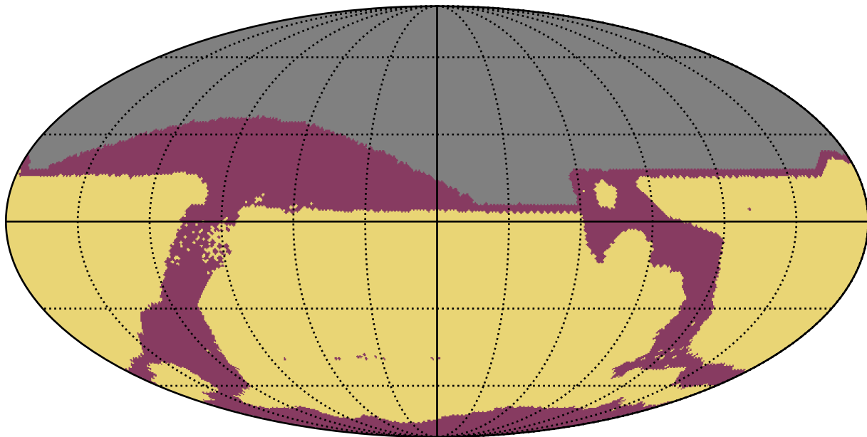
too_elab_r8_d2_griz_v3.4_10yrs : RapidRevisits
