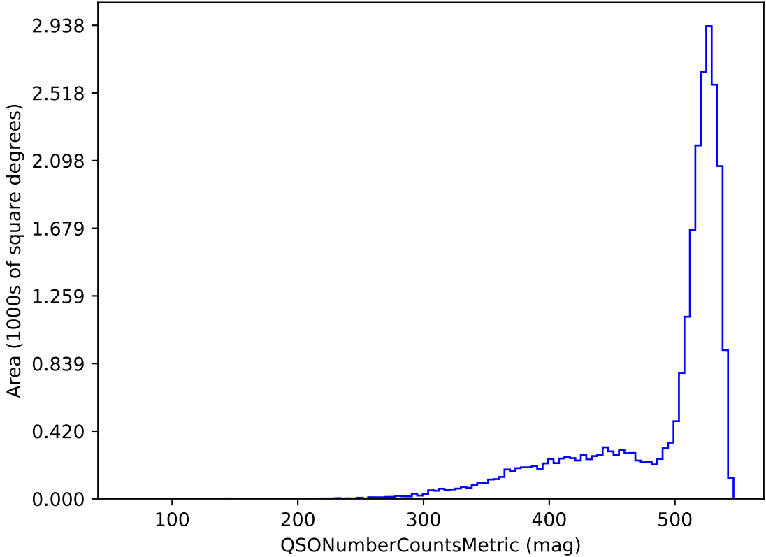
too_elab_r8_d2_griz_v3.4_10yrs r band and non-DD: QSONumberCountsMetric
