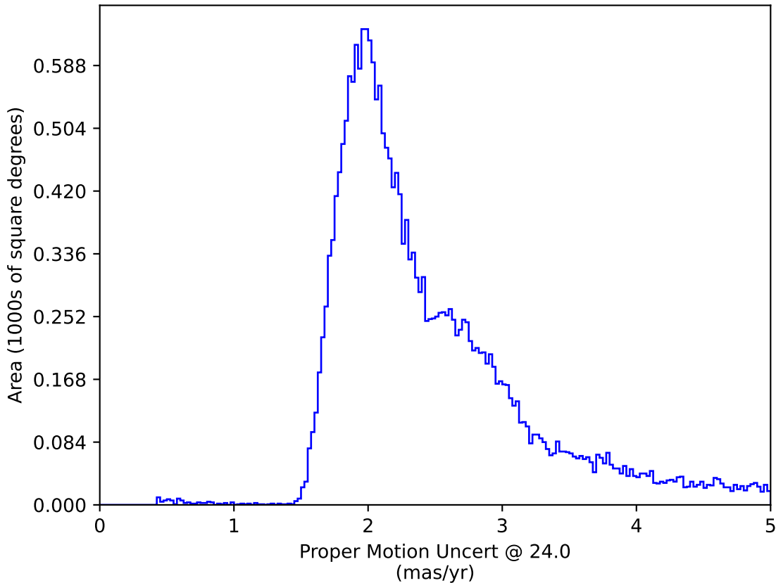
too_elab_r8_d2_griz_v3.4_10yrs : Proper Motion Uncert @ 24.0
