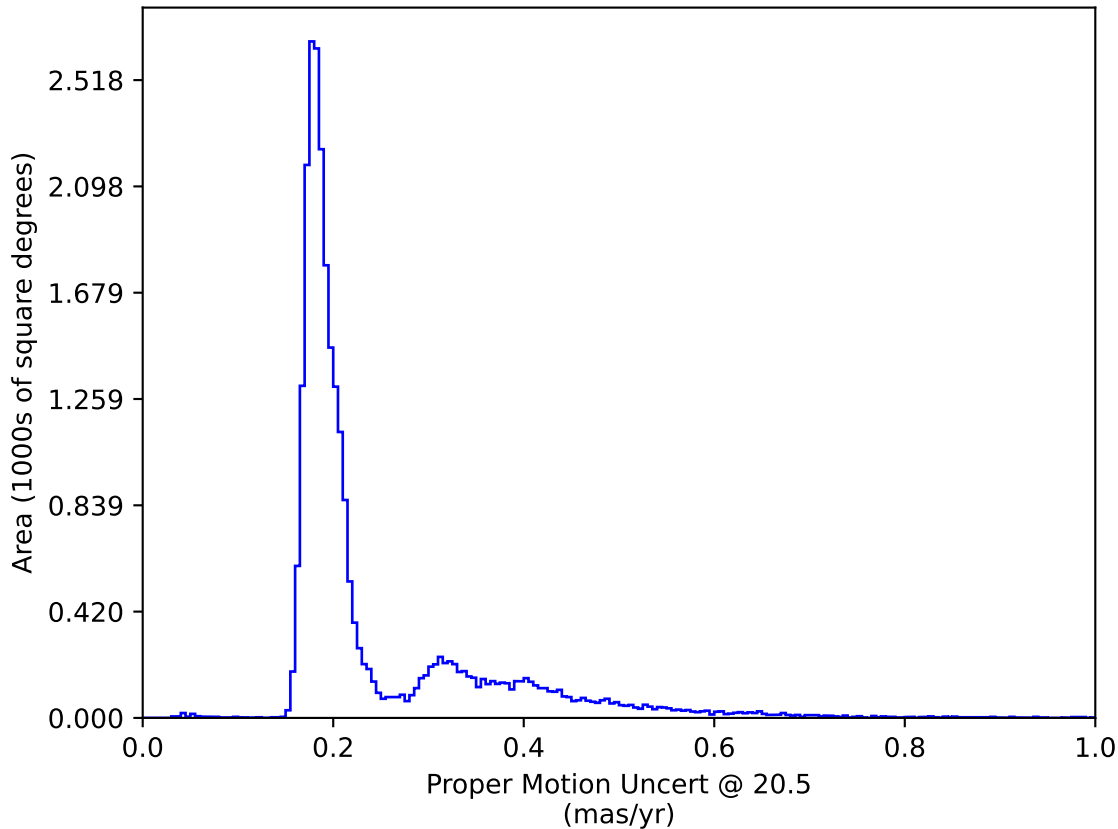
too_elab_r8_d2_griz_v3.4_10yrs : Proper Motion Uncert @ 20.5
