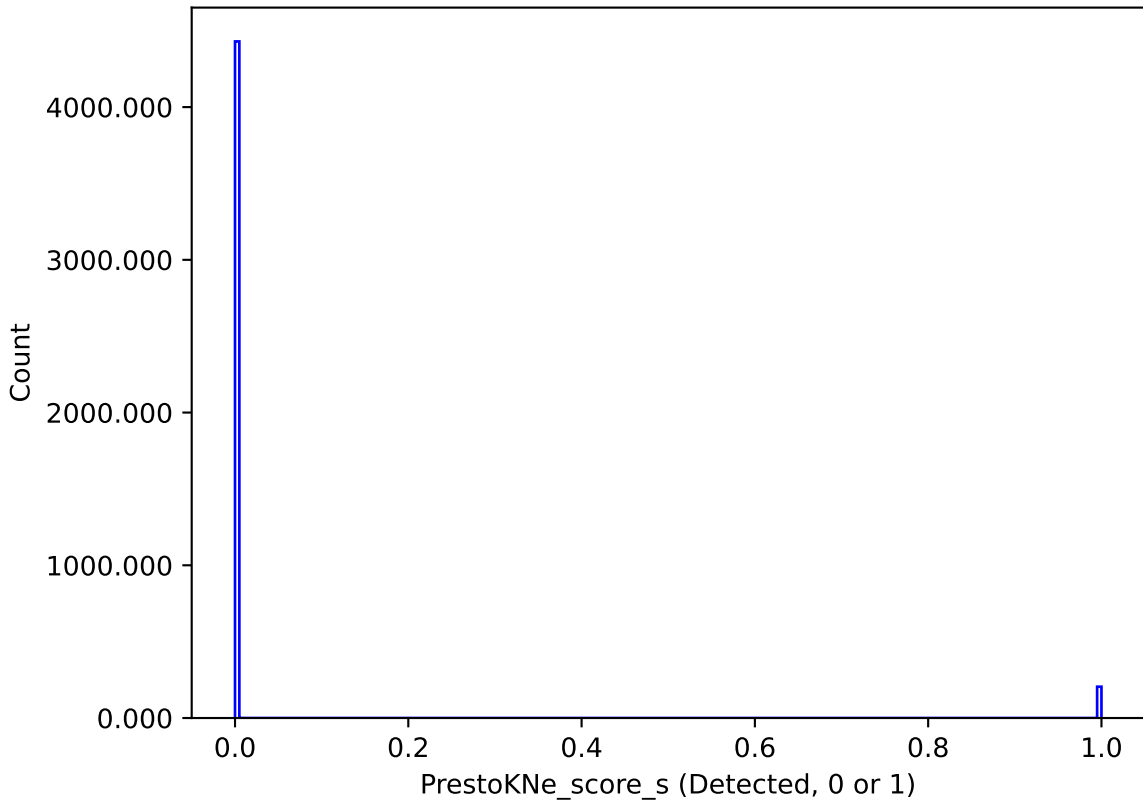
too_elab_r8_d2_griz_v3.4_10yrs : PrestoKNe_score_s
