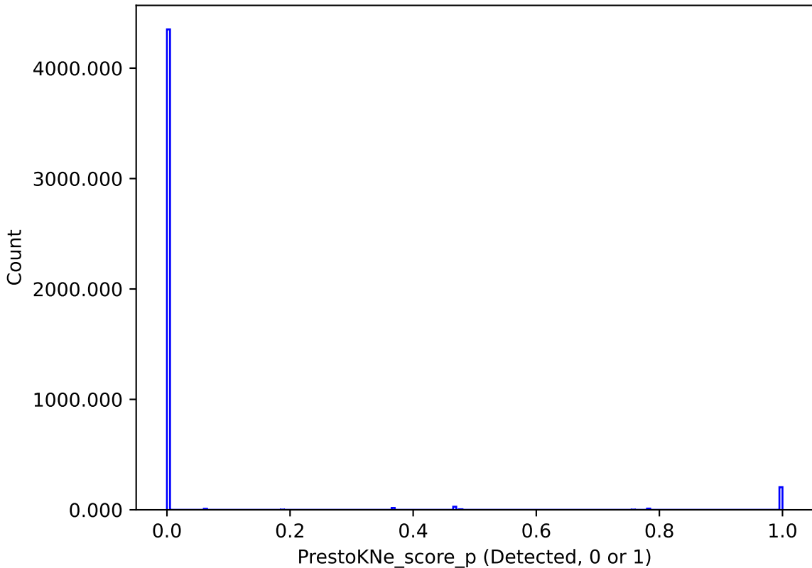
too_elab_r8_d2_griz_v3.4_10yrs : PrestoKNe_score_p
