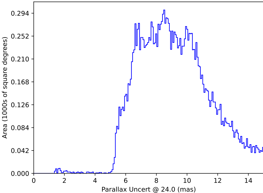
too_elab_r8_d2_griz_v3.4_10yrs : Parallax Uncert @ 24.0
