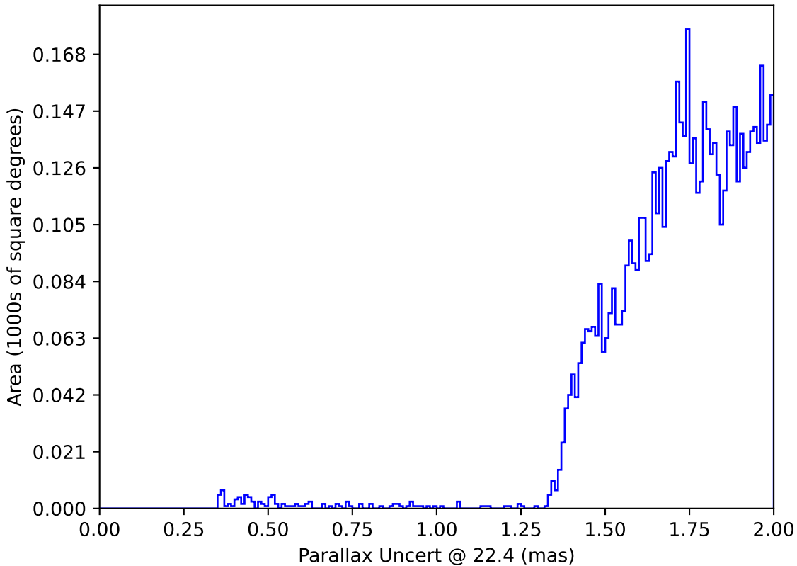
too_elab_r8_d2_griz_v3.4_10yrs : Parallax Uncert @ 22.4
