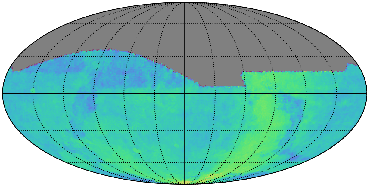
too_elab_r8_d2_griz_v3.4_10yrs : Parallax Coverage @ 24.0
