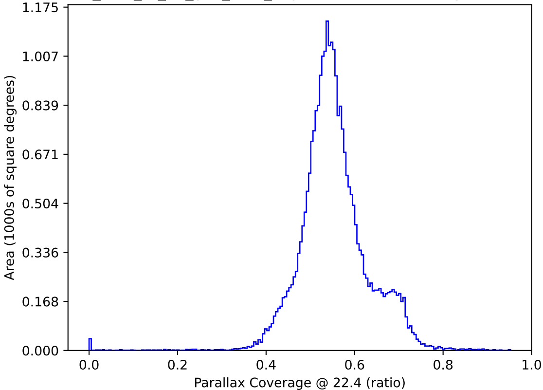
too_elab_r8_d2_griz_v3.4_10yrs : Parallax Coverage @ 22.4
