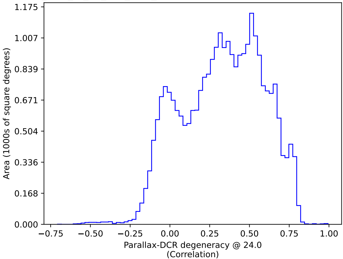
too_elab_r8_d2_griz_v3.4_10yrs : Parallax-DCR degeneracy @ 24.0
