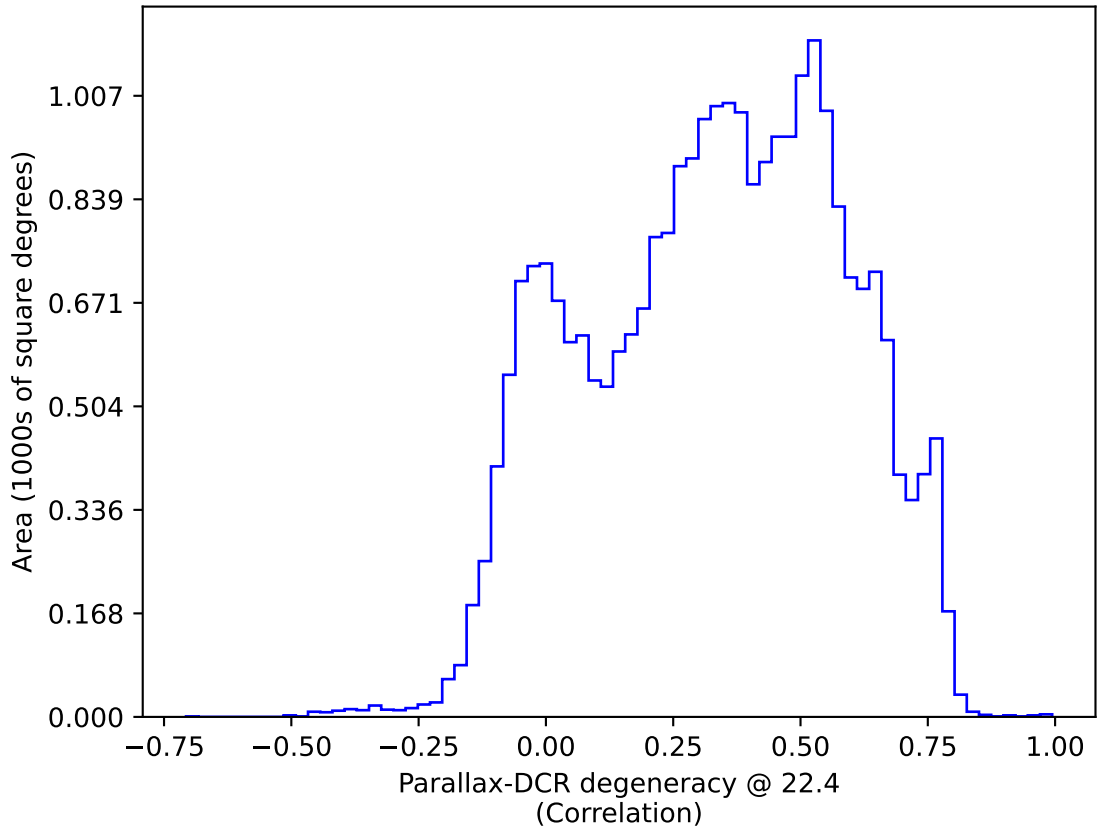
too_elab_r8_d2_griz_v3.4_10yrs : Parallax-DCR degeneracy @ 22.4
