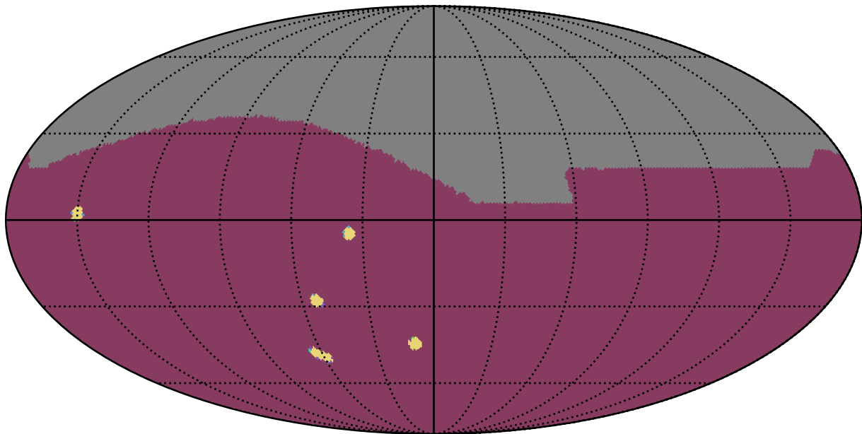
too_elab_r8_d2_griz_v3.4_10yrs : NumberOfQuickRevisits
